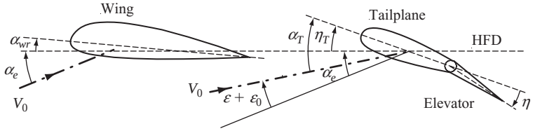
Figure 3.21 Practical wing–tailplane aerodynamic geometry.
