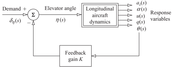
Figure 11.11 Longitudinal feedback options.
