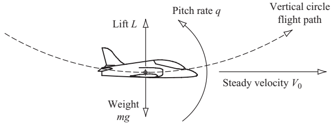
Figure 8.1 A symmetric pull-up manoeuvre.
