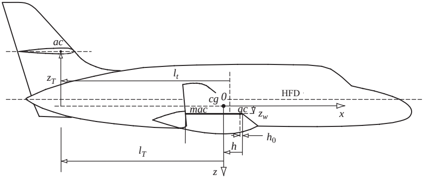
Figure 3.22 Practical aircraft longitudinal geometry.
